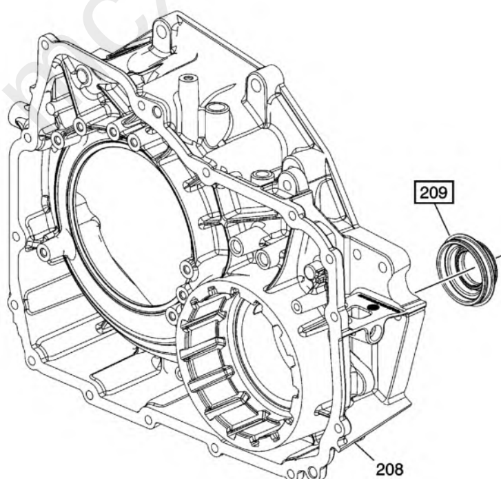
Fig. 2: Front Wheel Drive Shaft Seal Kit Components (Right Hand Side).(Gen 1 & 2)
