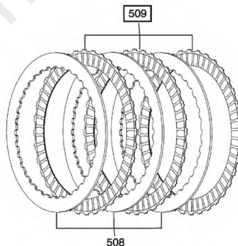
Fig. 15: 3-5 Reverse Plate Assembly Components (Gen 2) Courtesy of GENERAL MOTORS COMPANY
