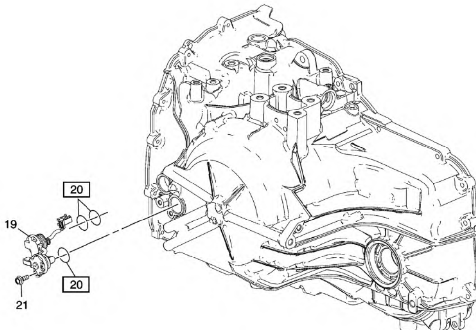
Fig. 1: Automatic Trans Seal Kit Components (Gen 1 And 2)
