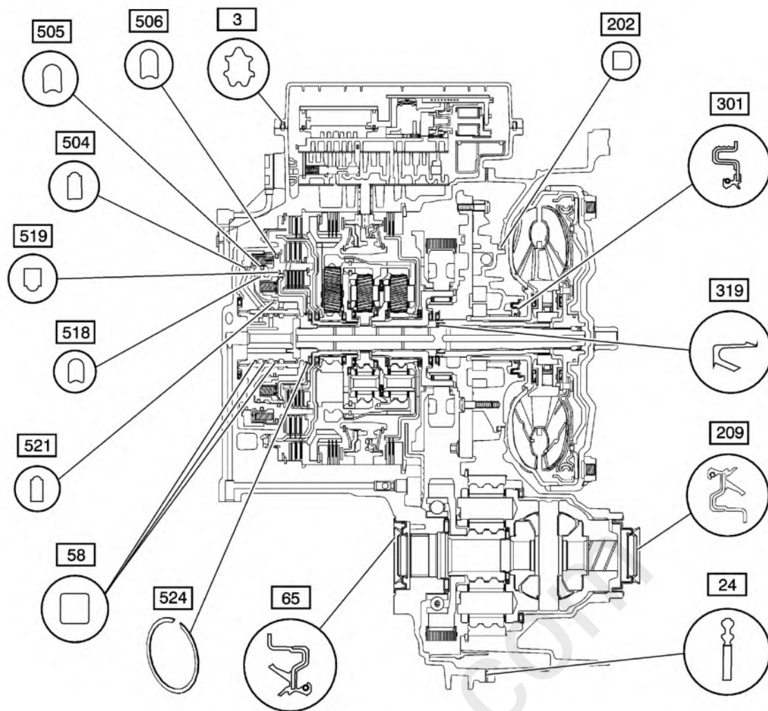
Fig. 6: Automatic Trans Seal Kit Components (Gen 2).(1 Of 2)
