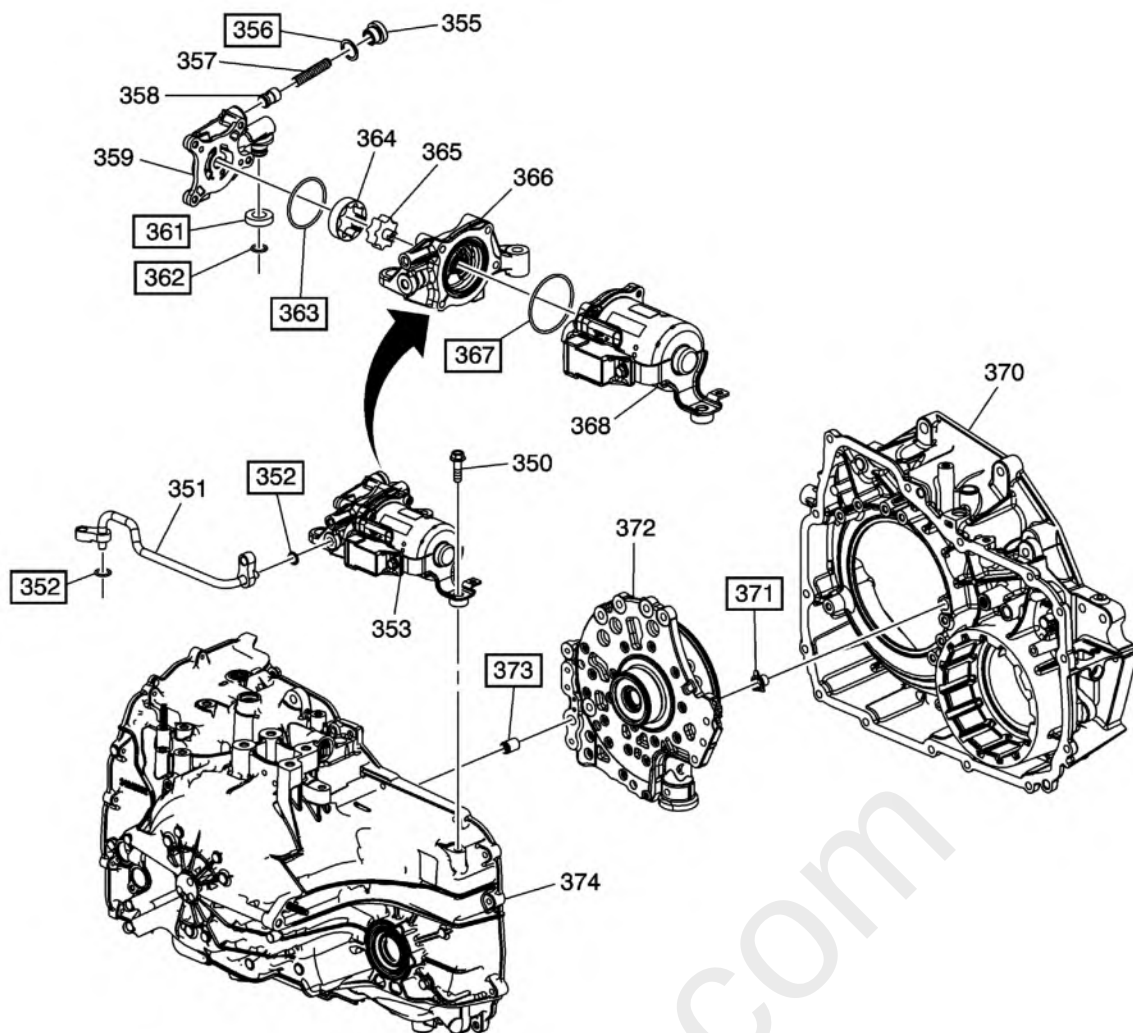
Fig. 18: Automatic Trans Seal Kit Components (Gen 2)
