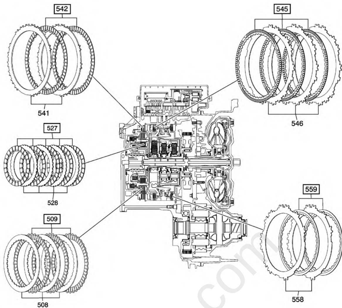
Fig. 12: Clutch Plate Package Components (Gen 2)
