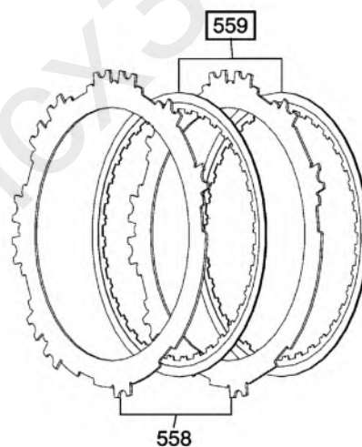
Fig. 17: 1-2-3-4 Plate Assembly Components (Gen 2)
