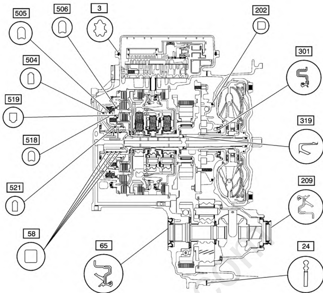
Fig. 4: Automatic Trans Seal Kit Components (Gen 1).(1 Of 2)
