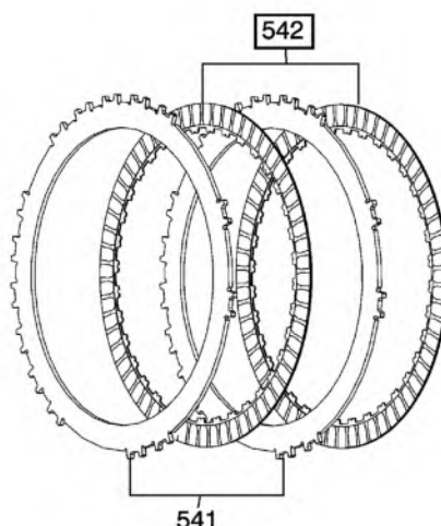
Fig. 16: 2-6 Plate Assembly Components (Gen 2)
