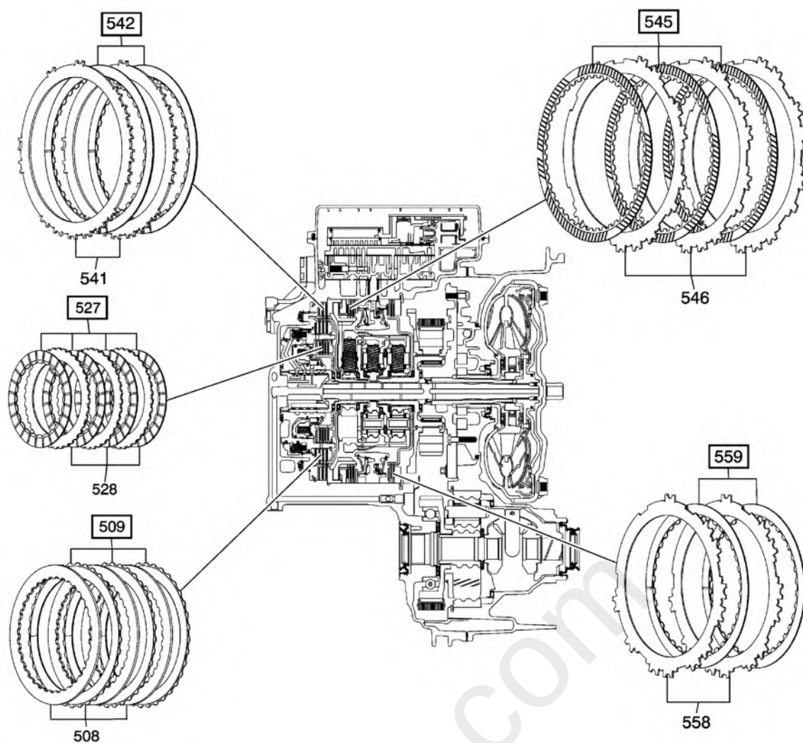
Fig. 11: Clutch Plate Package Components (Gen 1)
