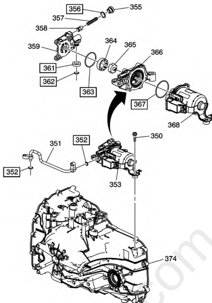
Fig. 19: Automatic Trans Auxiliary Seal Kit Components (Gen 2)
