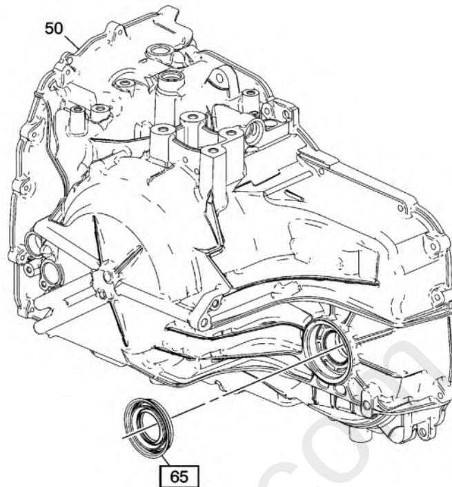
Fig. 3: Front Wheel Drive Shaft Seal Kit Components (Left Hand Side) (Gen 1 & 2)
