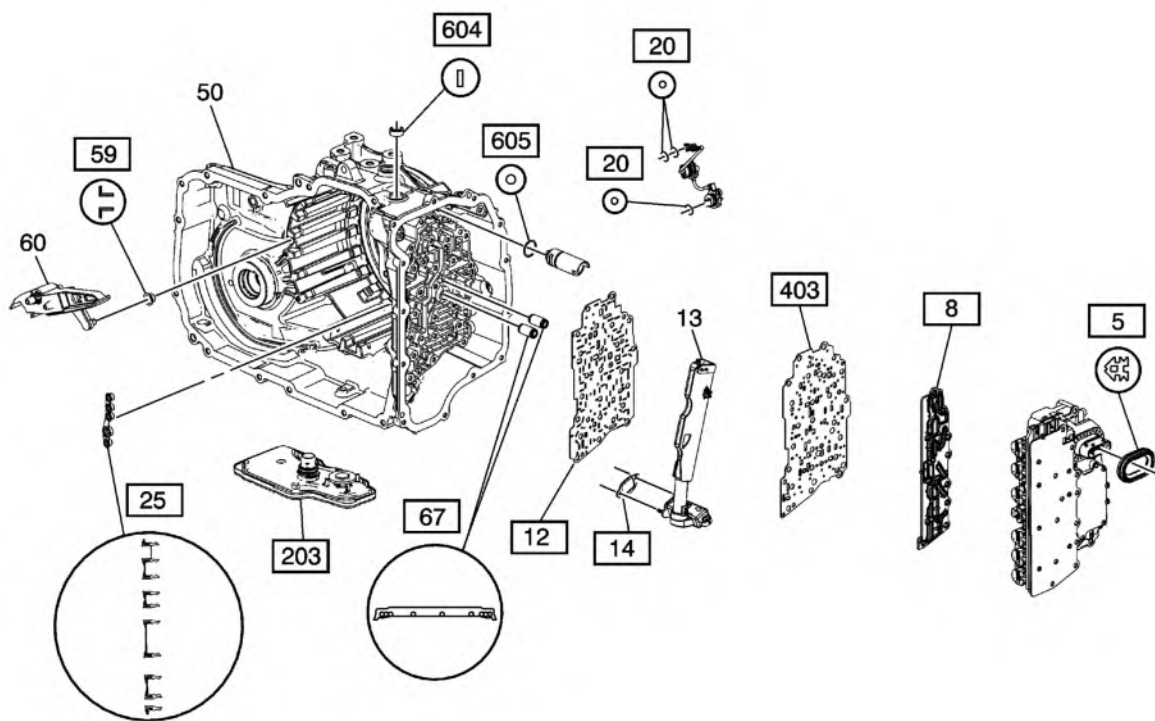
Fig. 5: Automatic Trans Seal Kit Components (Gen 1).(2 Of 2)
