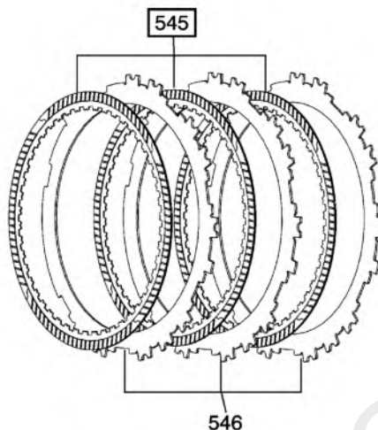
Fig. 14: Low And Reverse Plate Assembly Components (Gen 2) Courtesy of GENERAL MOTORS COMPANY
