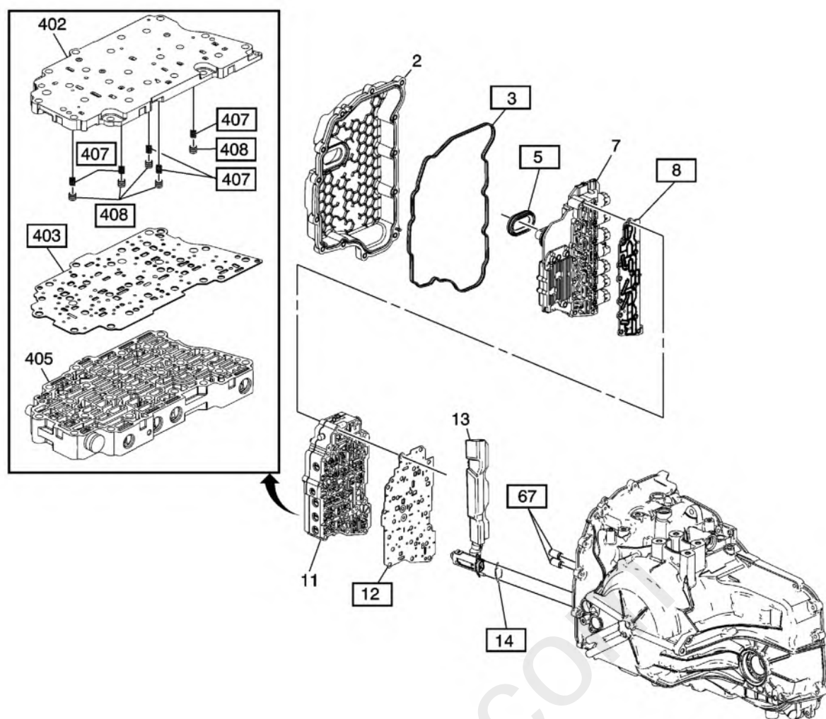
Fig. 10: Control Valve Body Kit Components (Gen 2).
