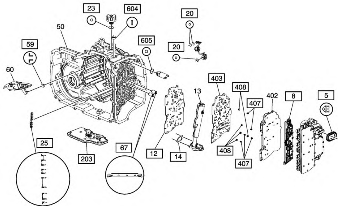
Fig. 7: Automatic Trans Seal Kit Components (Gen 2).(2 Of 2)
